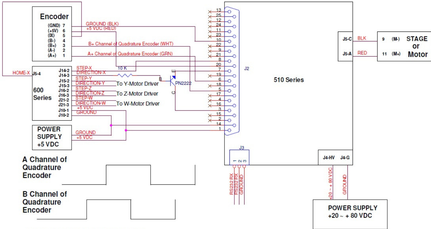
CBL-02 Wiring Diagram
